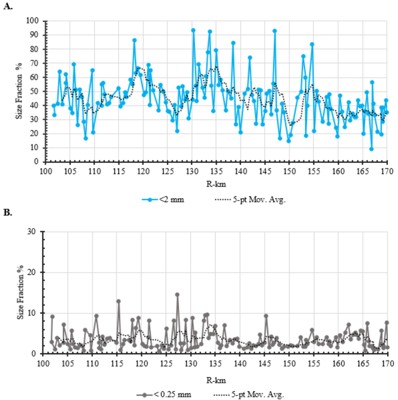
Figure 21: Downstream size trends in gravel bar bulk percentages for fine sediments. A. <2 mm. B. <0.25 mm.
