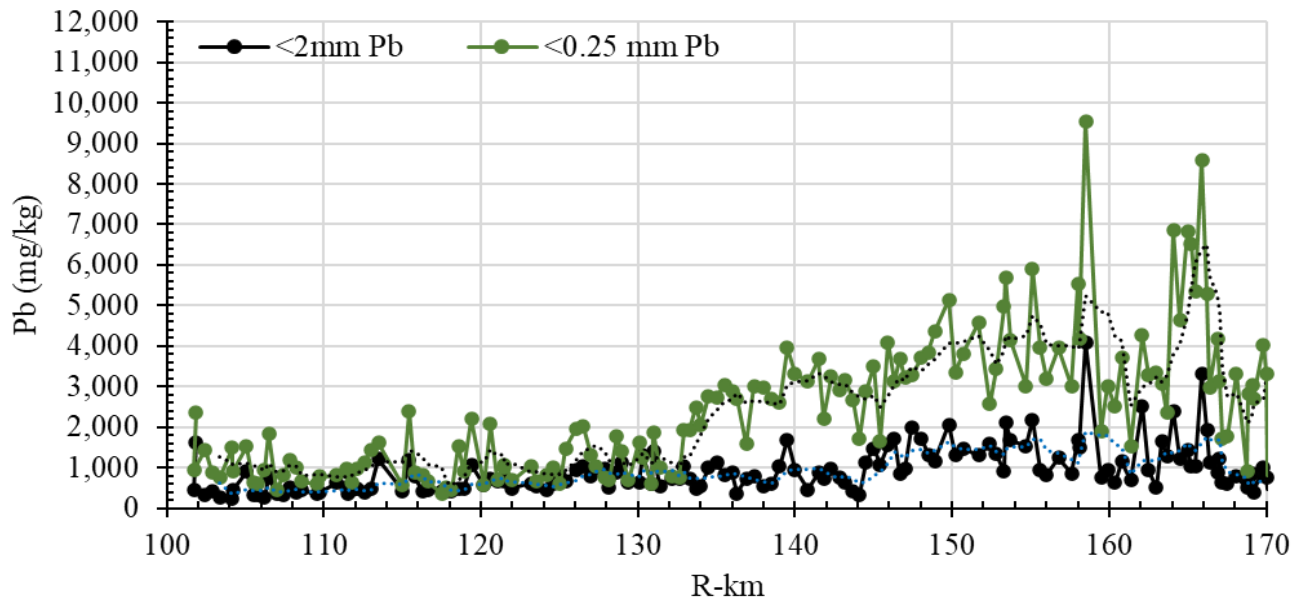
Figure 31: Pb in <2 and <0.25 mm Big River bar sediments. Moving average (5-pt) is shown as dotted line. PEC limit for Pb is 128 mg/kg.
