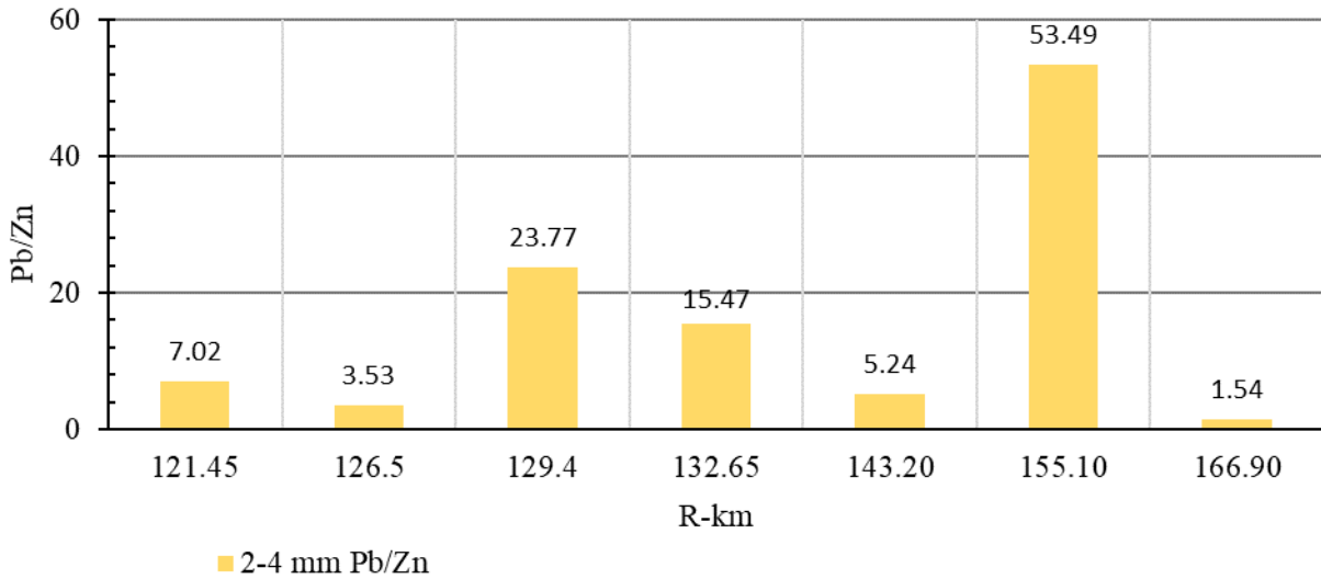
Figure 43: Chat grain Pb/Zn ratios by R-km. A. 4-8 mm and B. 2-4 mm coarse dolomite grains from gravel bar samples. Pb/Zn ratios are unique for different chat piles and can be used to identify contaminant source.
