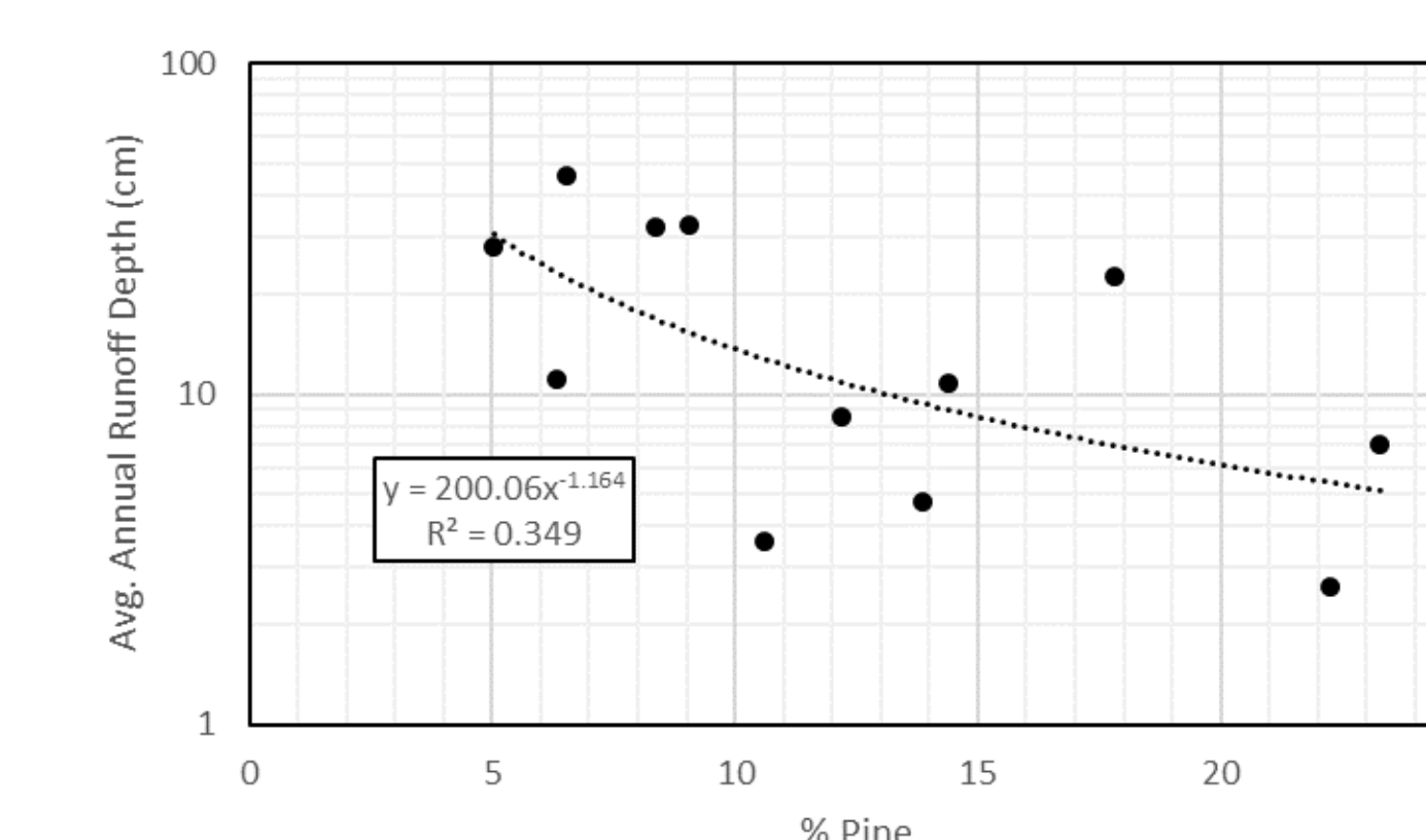
Figure 11. Average annual runoff depth vs. % pine within the watershed from water years 2016-2020 at Big Barren Creek.
