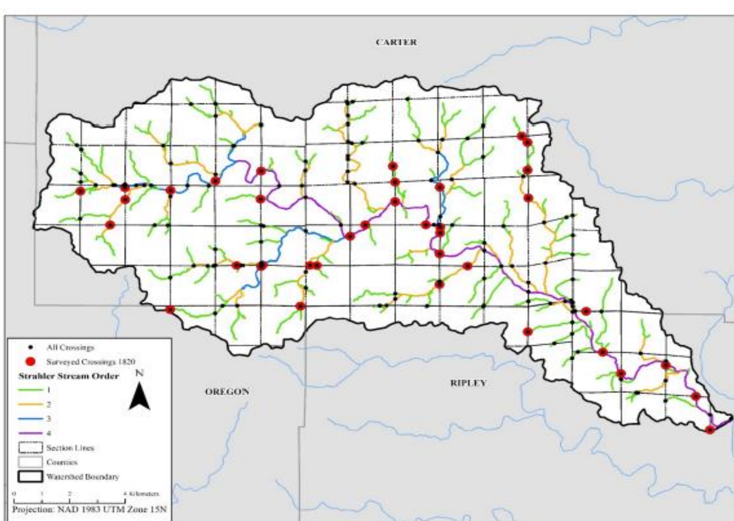
Figure 6. Locations of sites in the watershed where GLO surveyors recorded channel width in field notes in 1821.
