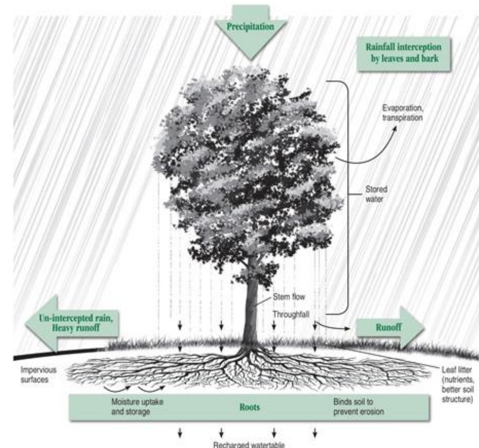
Figure 1. The role of trees in hydrology. ( https://treecanopybmp.org )
