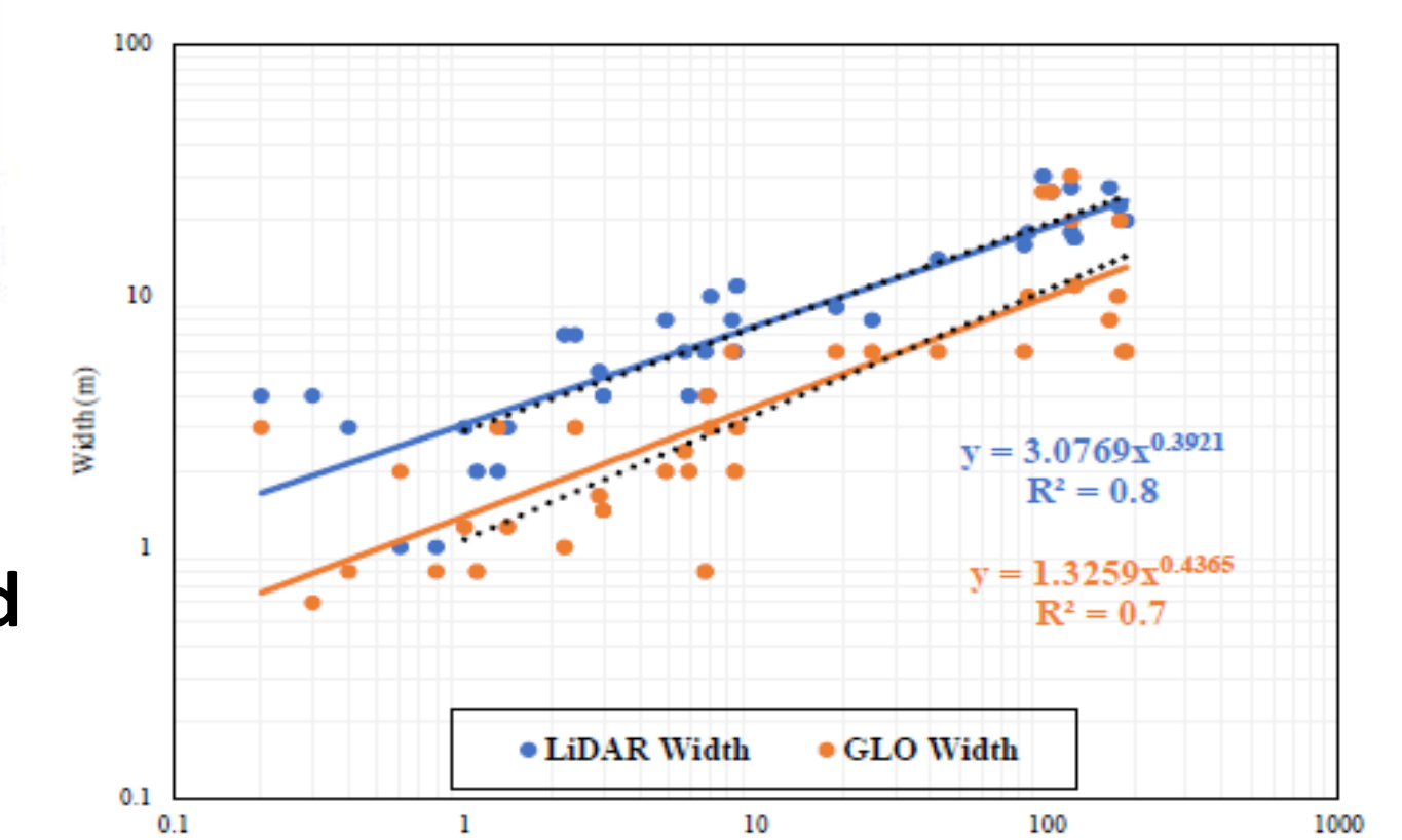
Figure 7. GLO recorded width from 1821 compared to modern LiDAR derived width.
