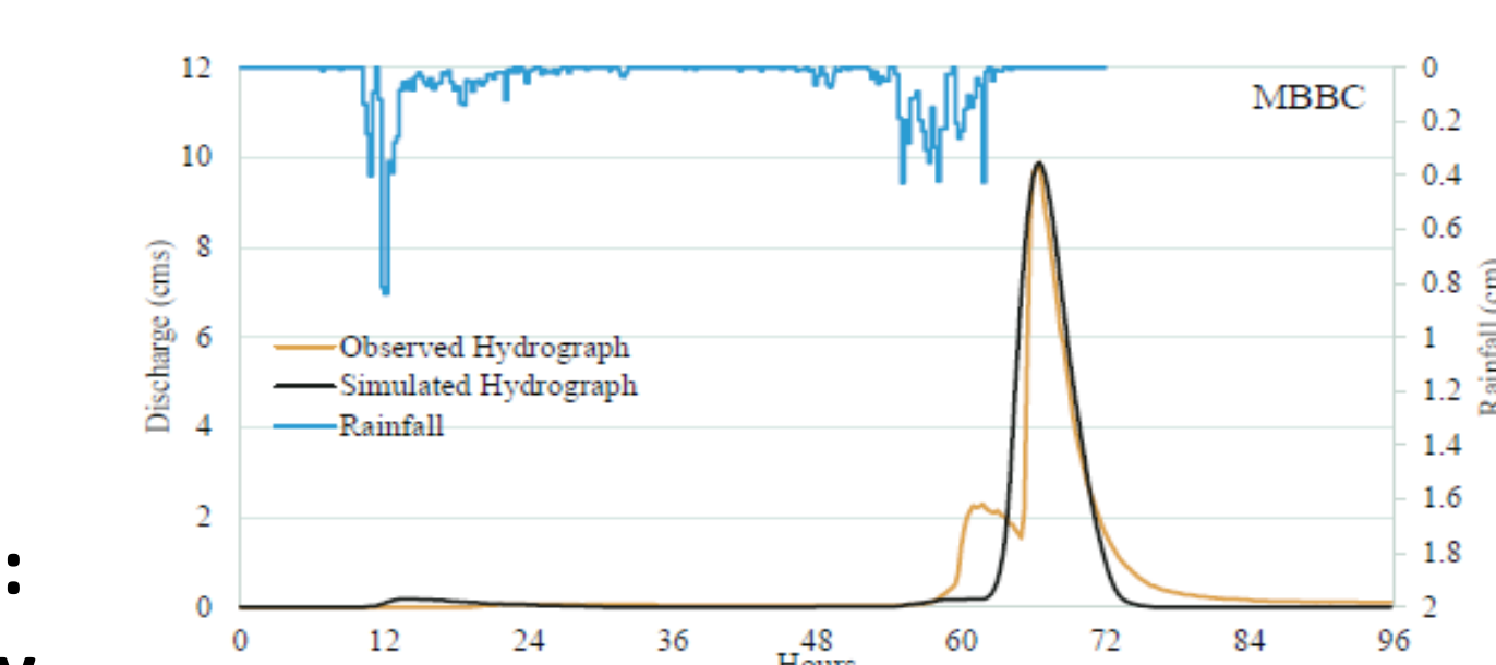
Figure 9. Simulated and observed hydrograph and rainfall.
