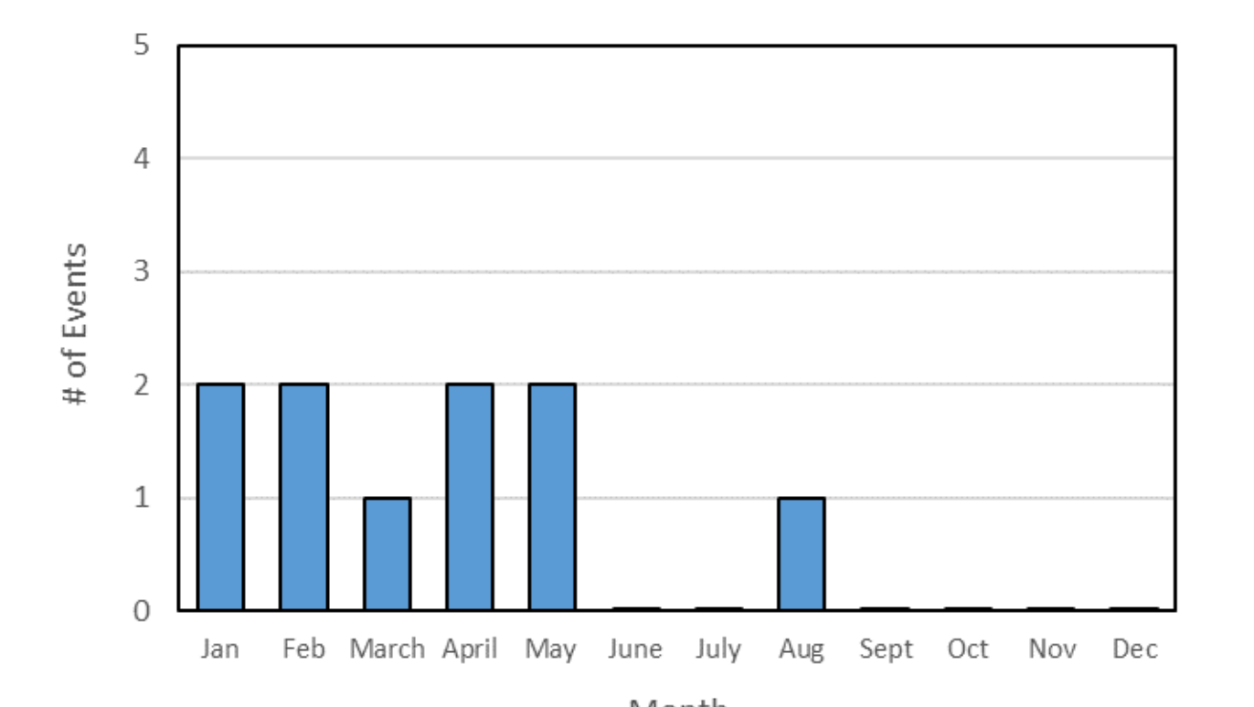
Figure 12. Number of significant flood events in Big Barren Creek from water year 2016-2021.
