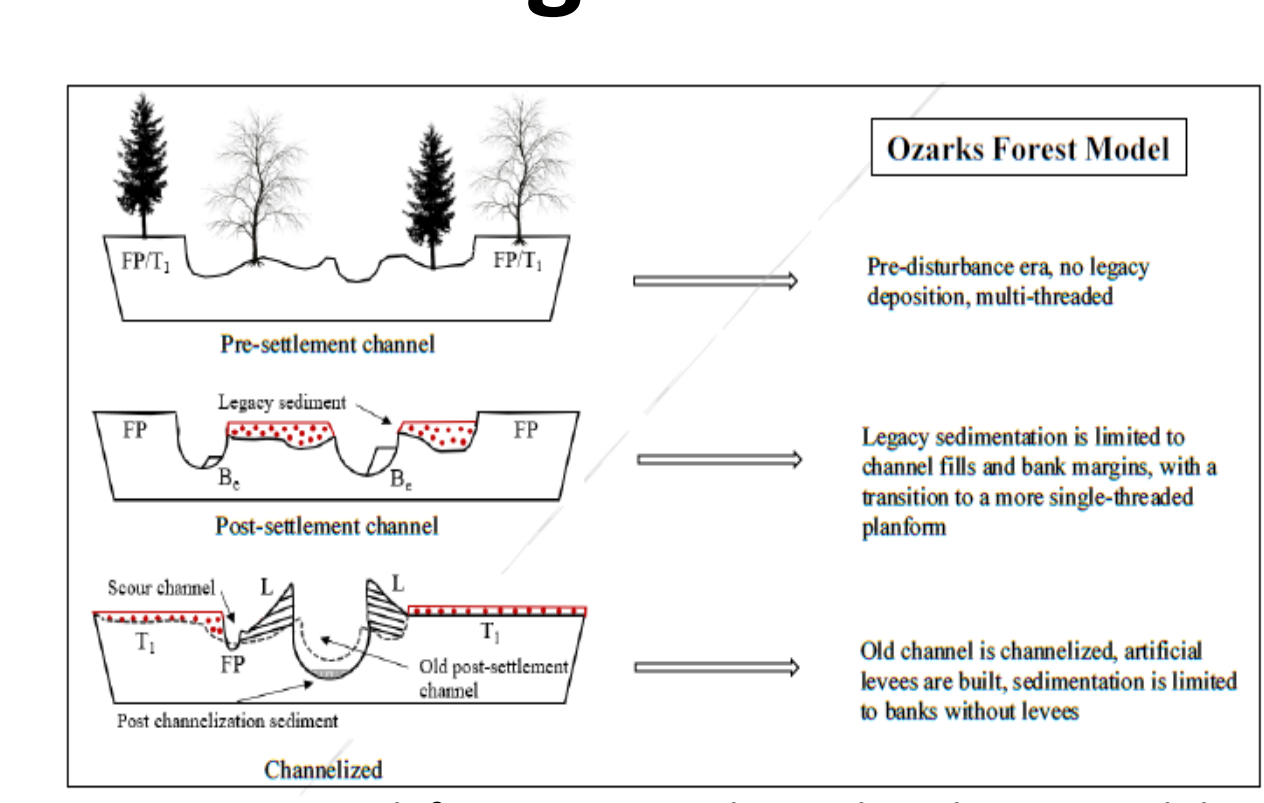
Figure 10. Ozark forest stream channel evolution model showing the pre-settlement, multi-threaded channel transition to a single threaded channel today (Reminga 2019).
