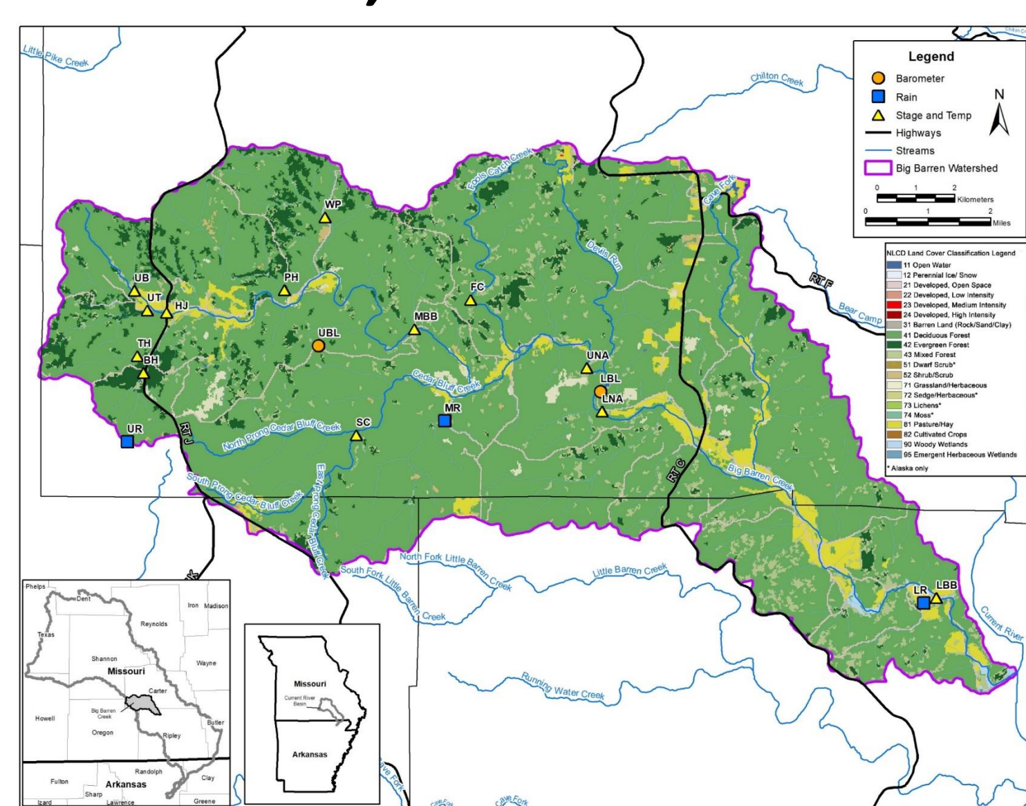
Figure 3. 2016 land use of Big Barren Creek watershed.
