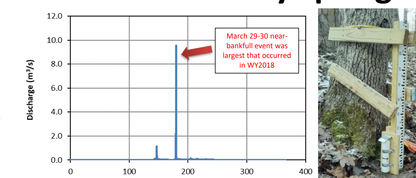
Figure 8. Annual hydrograph for WY2018 showing only two significant flood events over the year. Photo shows an example of gaging station installed in sub-basins within the watershed.
