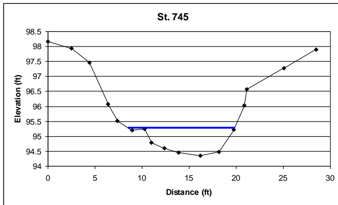
Figure 4a: Cross-section in Subreach #1.
